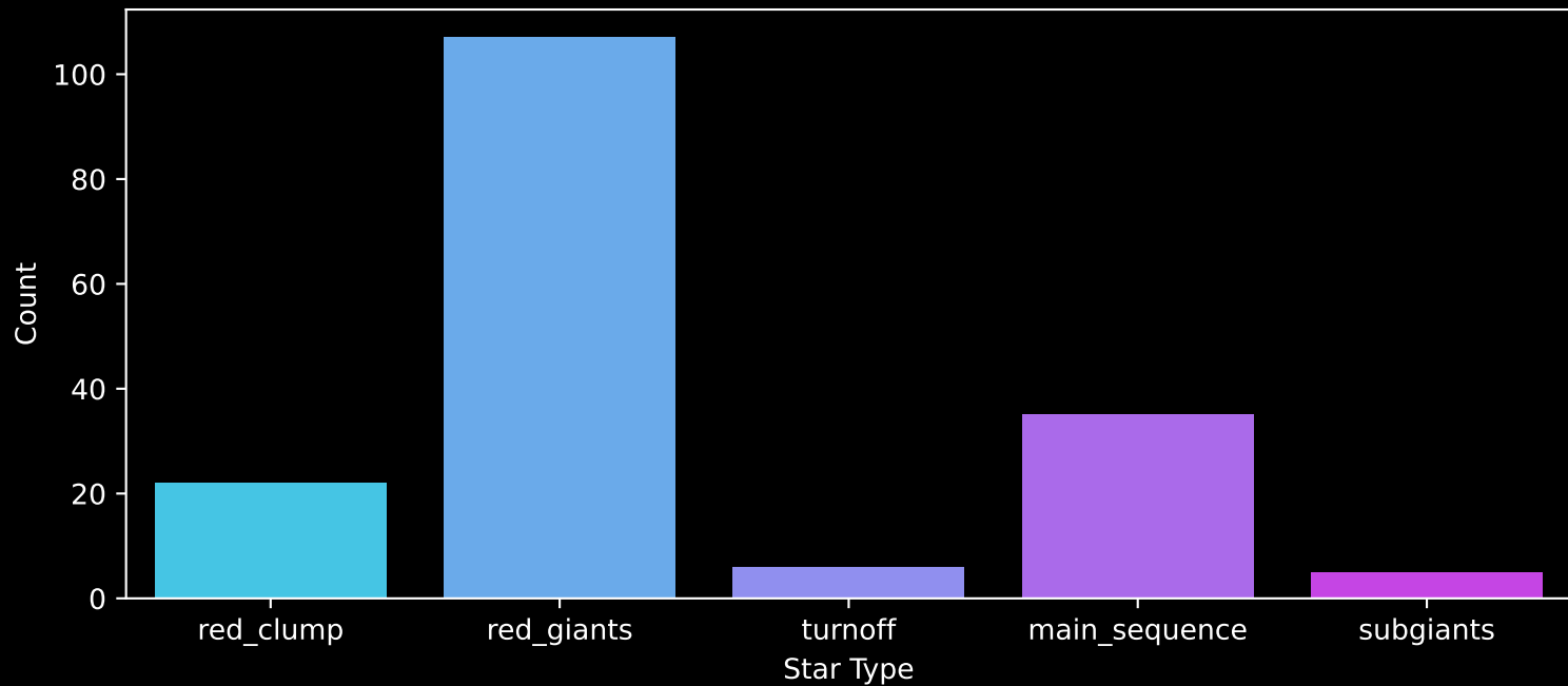
APOGEE DR17 Field: [203+21] Count plot of Star Type
