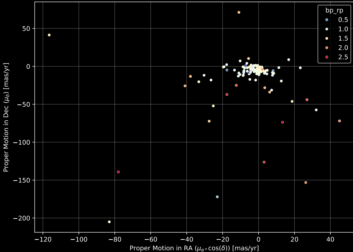
APOGEE DR17 Field: [203+21] Proper Motion Diagram (n= 175)
