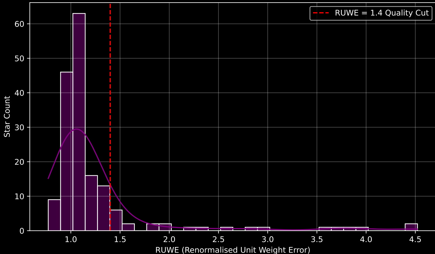
GAPOGEE DR17 Field [203+21] RUWE Distribution (n= 170)
