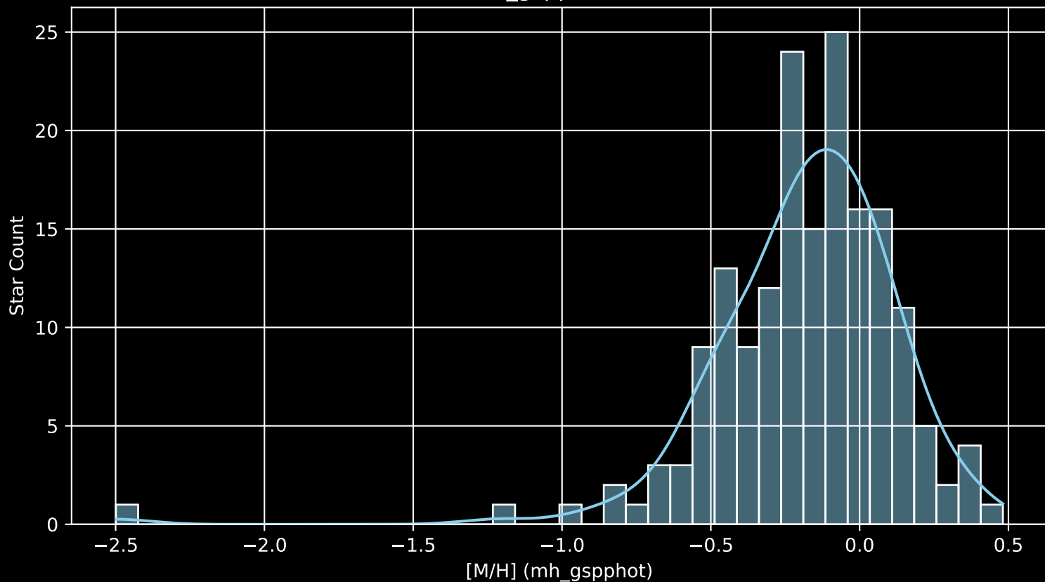
APOGEE DR17 Field: [203+21 [M/H] (mh_gspphot) (n= 174)
