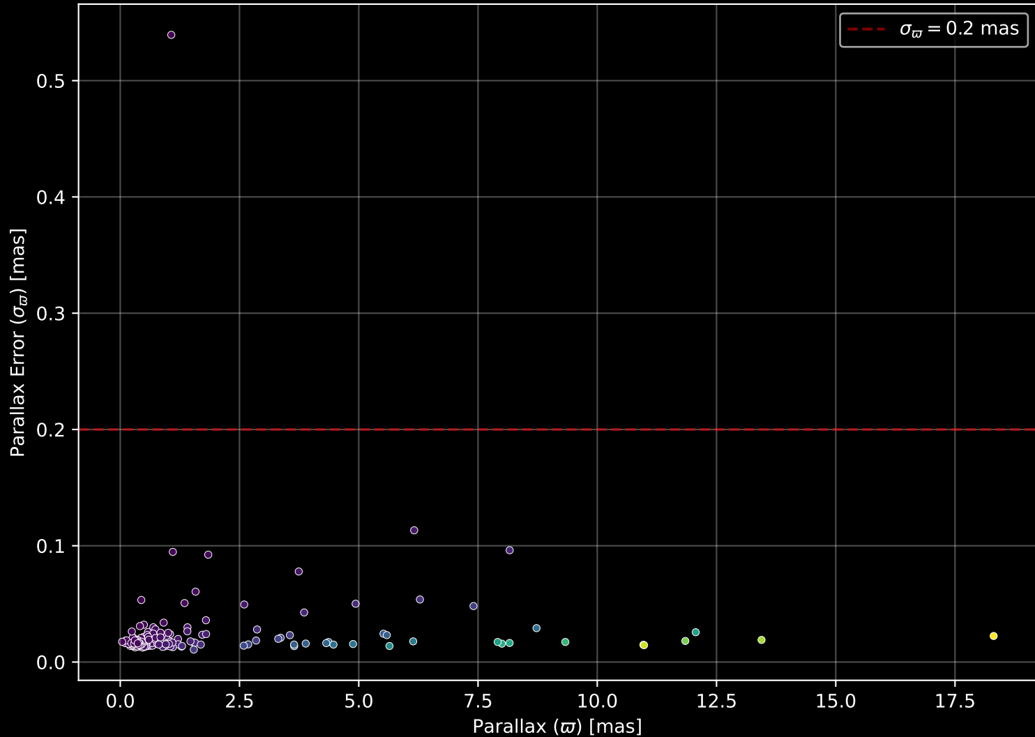
APOGEE DR17 Field: [203+21] Parallax Quality (n= 175)
