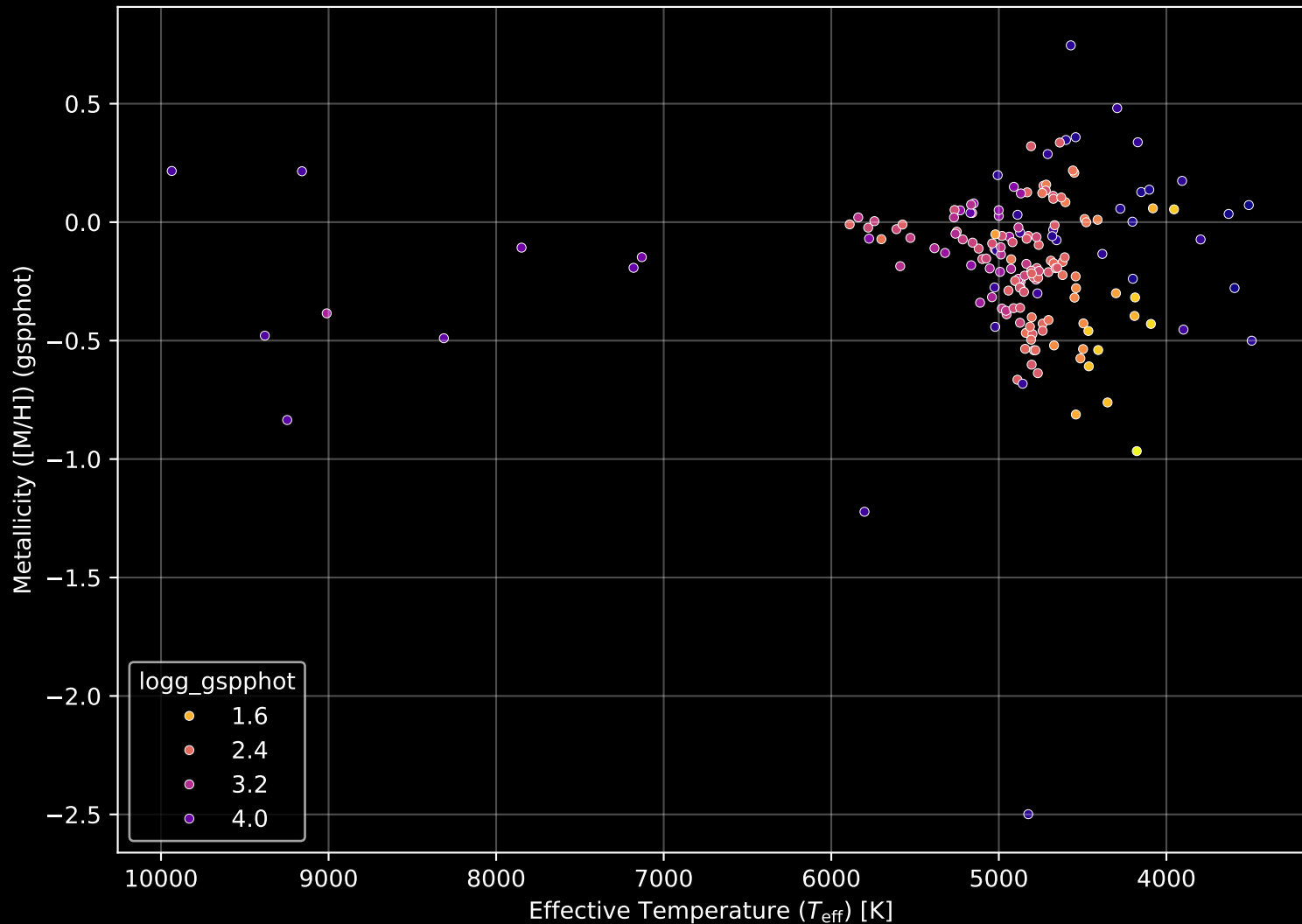
APOGEE DR17 Field: [203+21] Stellar Population Parameters (n= 175)
